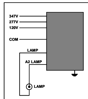
Wiring Diagram
